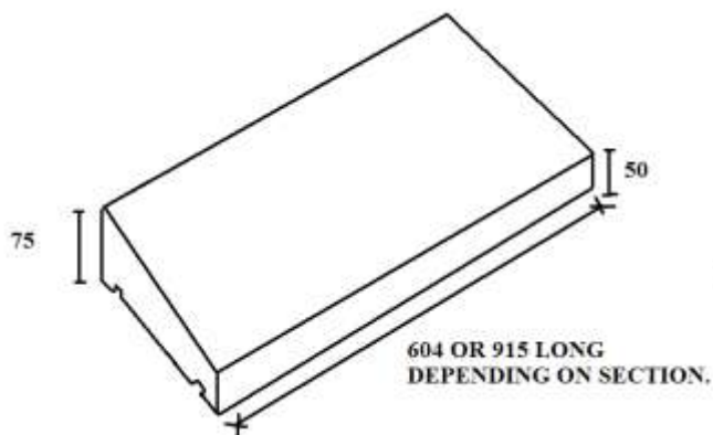
ONCE WEATHERED COPING (O/W)
