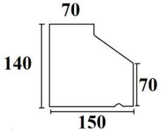
150 X 140 MM HIGH
