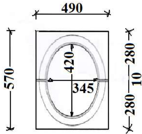
SMALL OVAL WINDOW.
