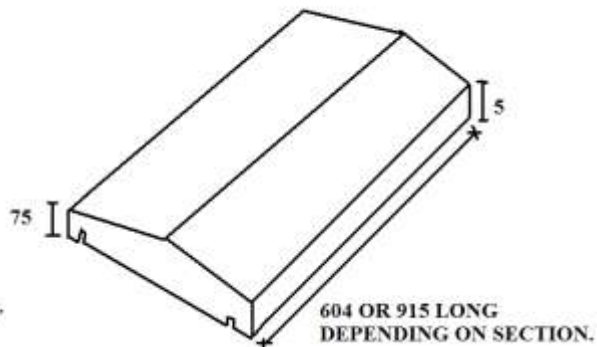
TWICE-WEATHERED COPING (T/W)
