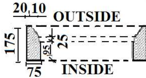
TYPICAL SECTION.
